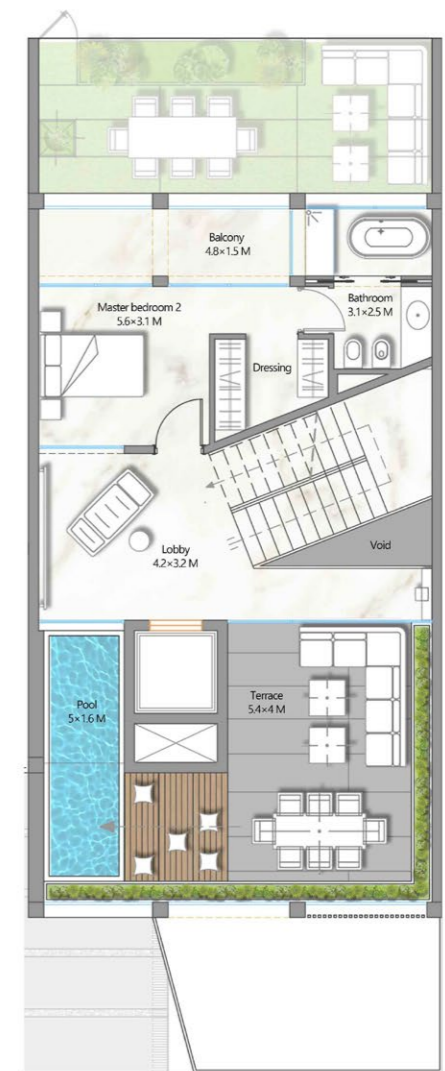
ROOF FLOOR PLAN
